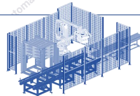
Robot palletizer
